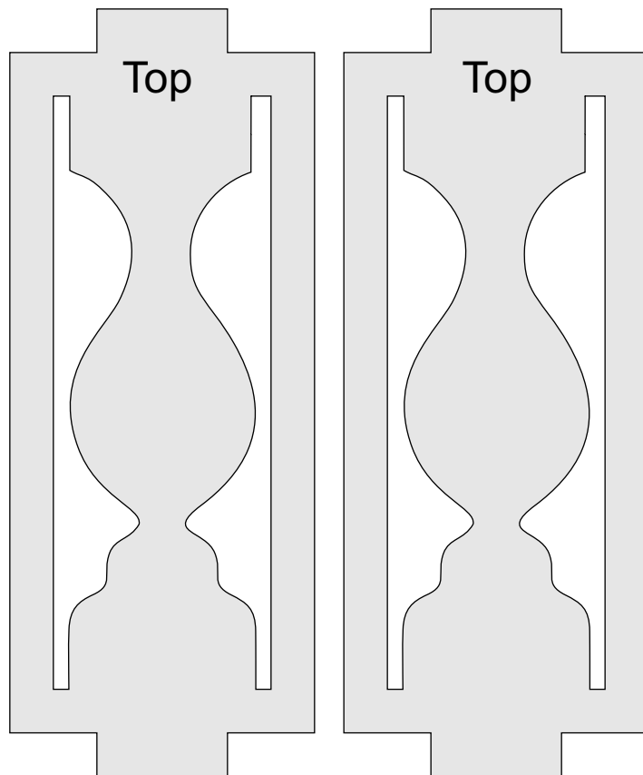
45 Degree Ends
